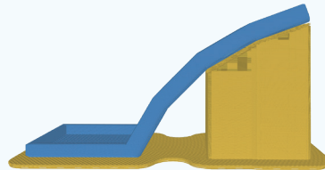
an overhang angle of 60^\circ
